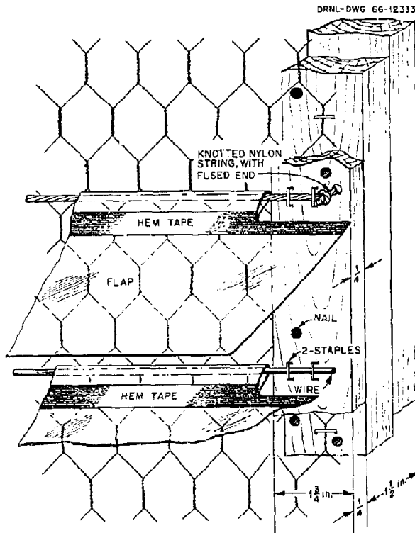
Fig. B-13. Mesh wire stops
